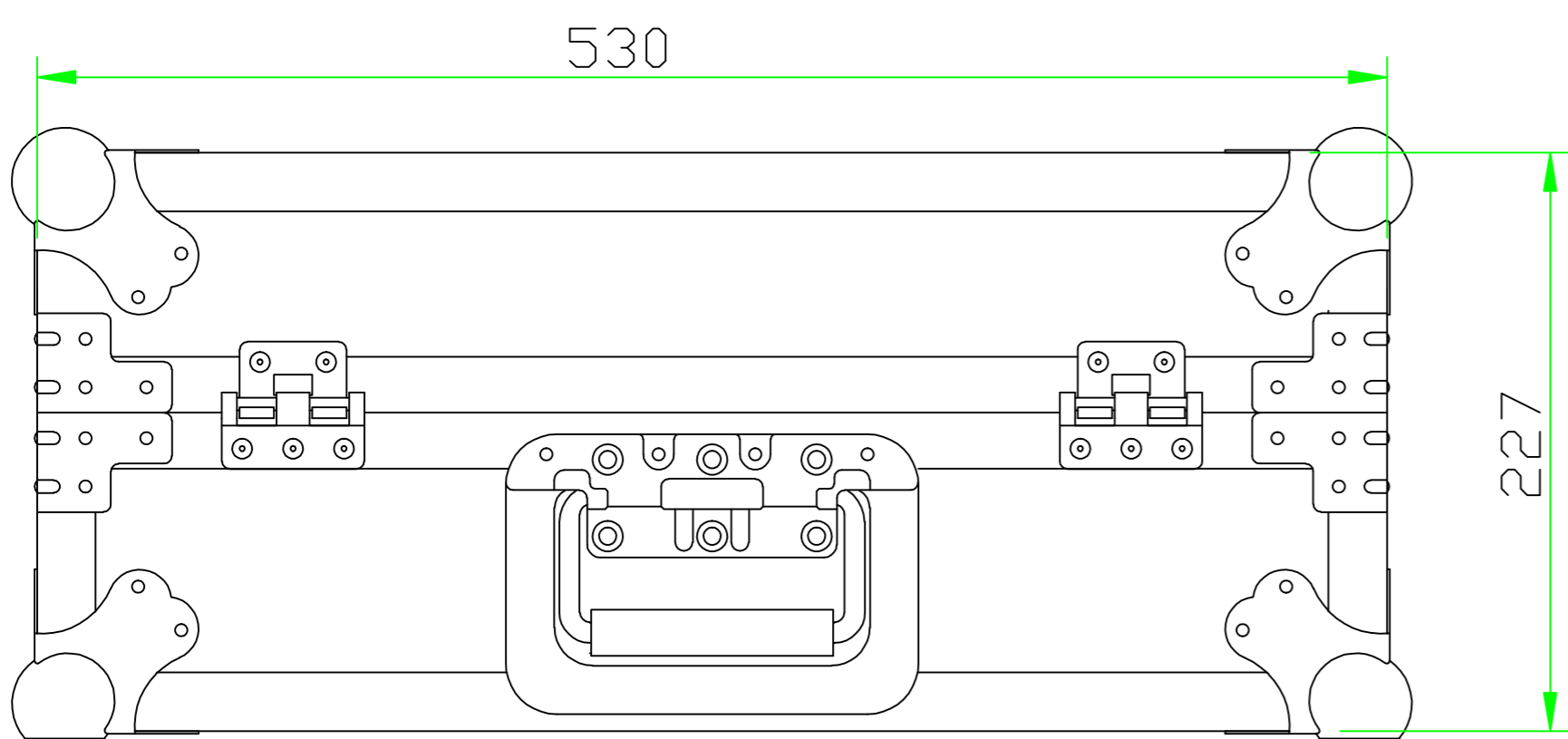
BACK VIEW
