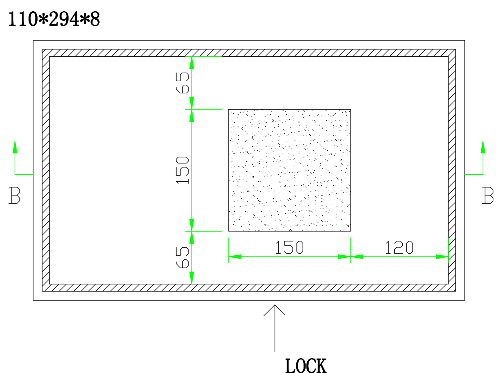
INSIDE VIEW OF COVER
