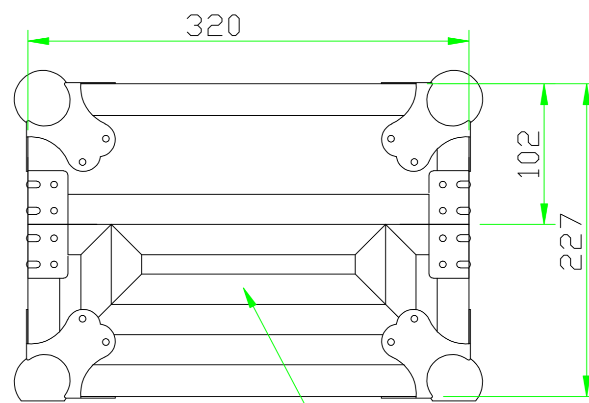
LEFT VIEW
