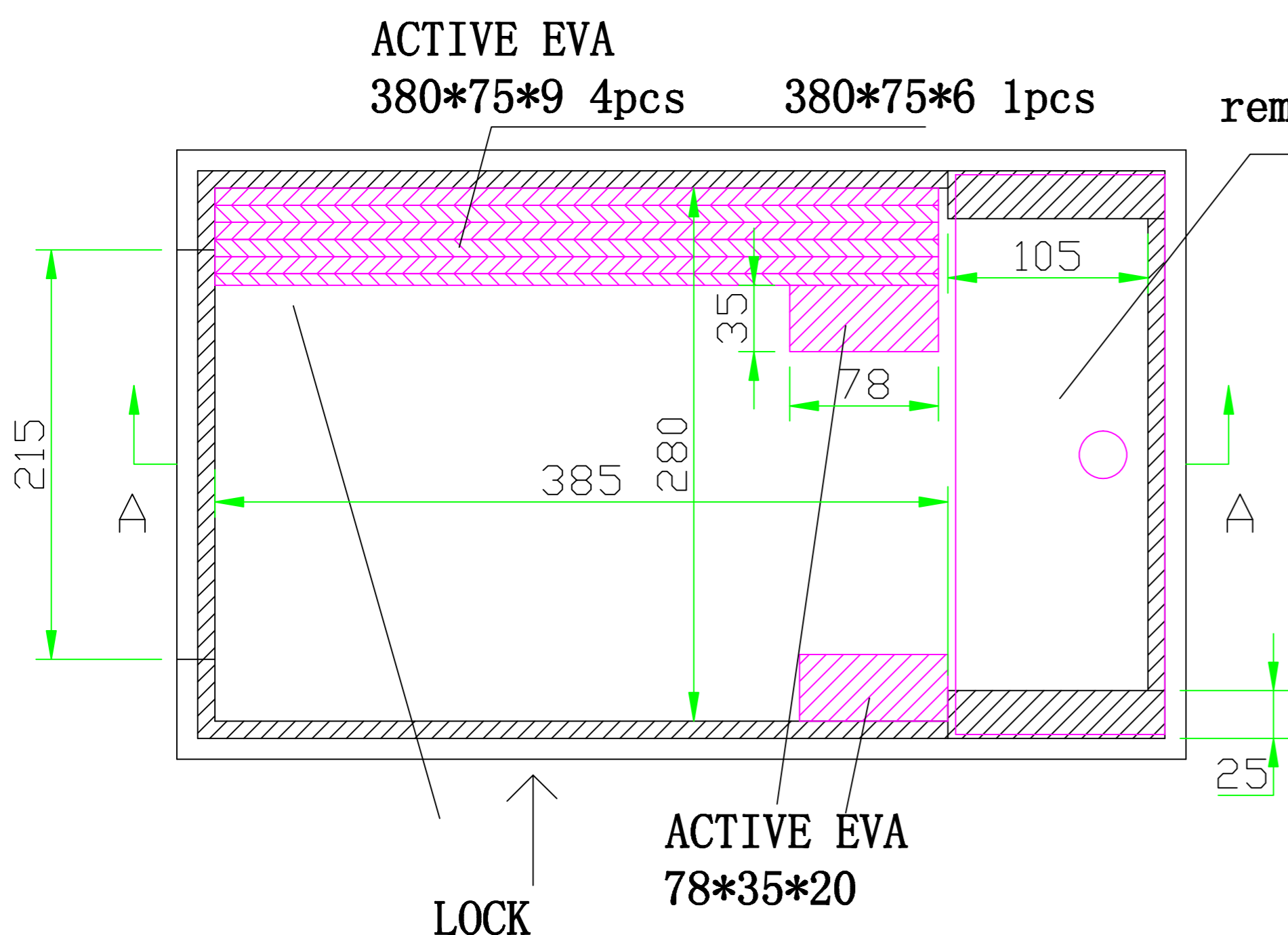
INSIDE VIEW OF BASE
