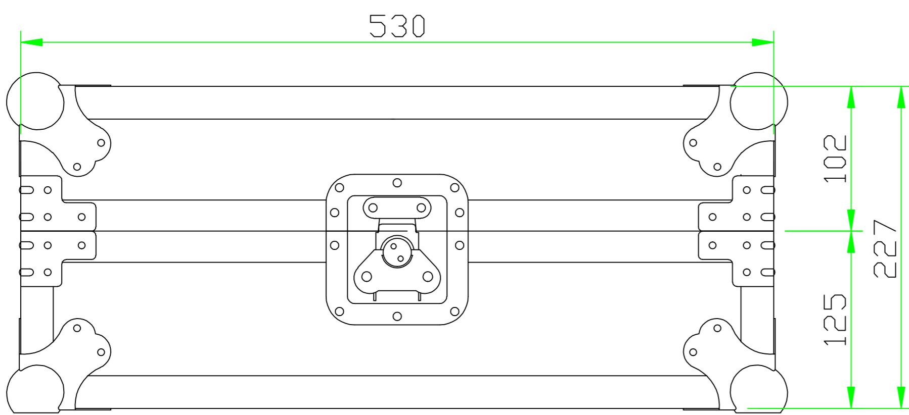
FRONT VIEW
