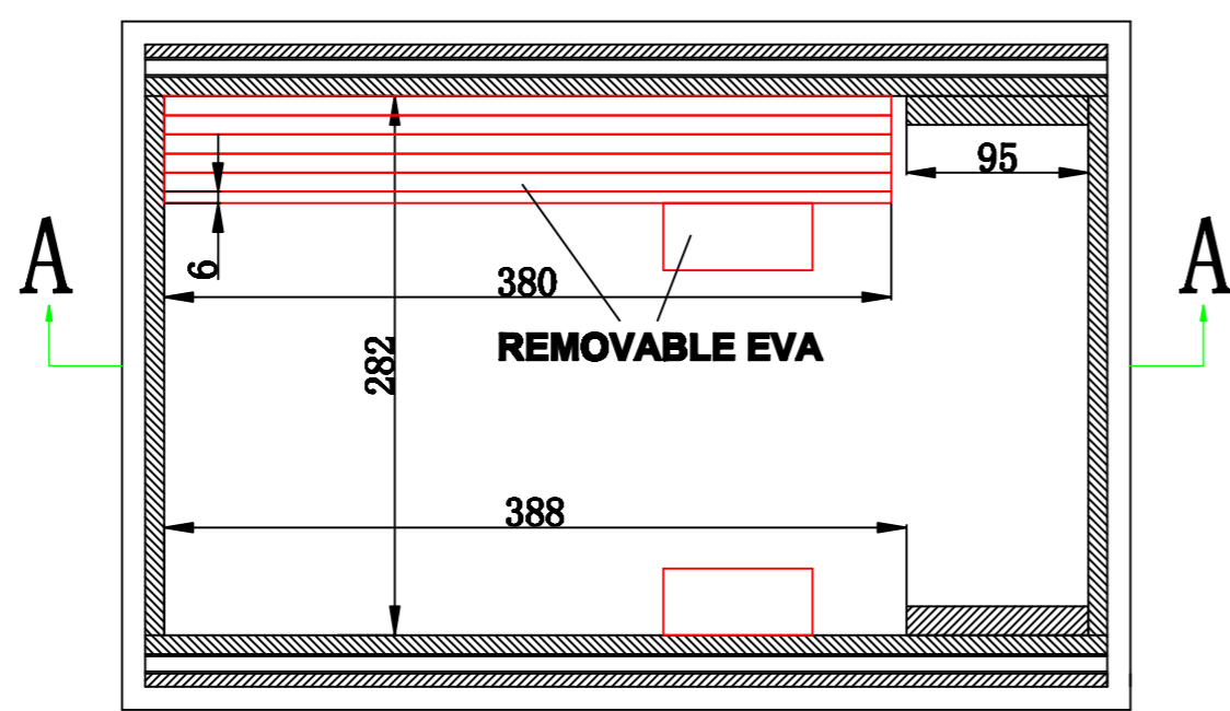
INSIDE VIEW OF BASE
