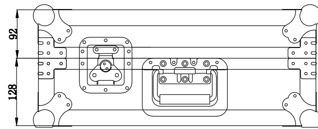
RIGHT VIEW
