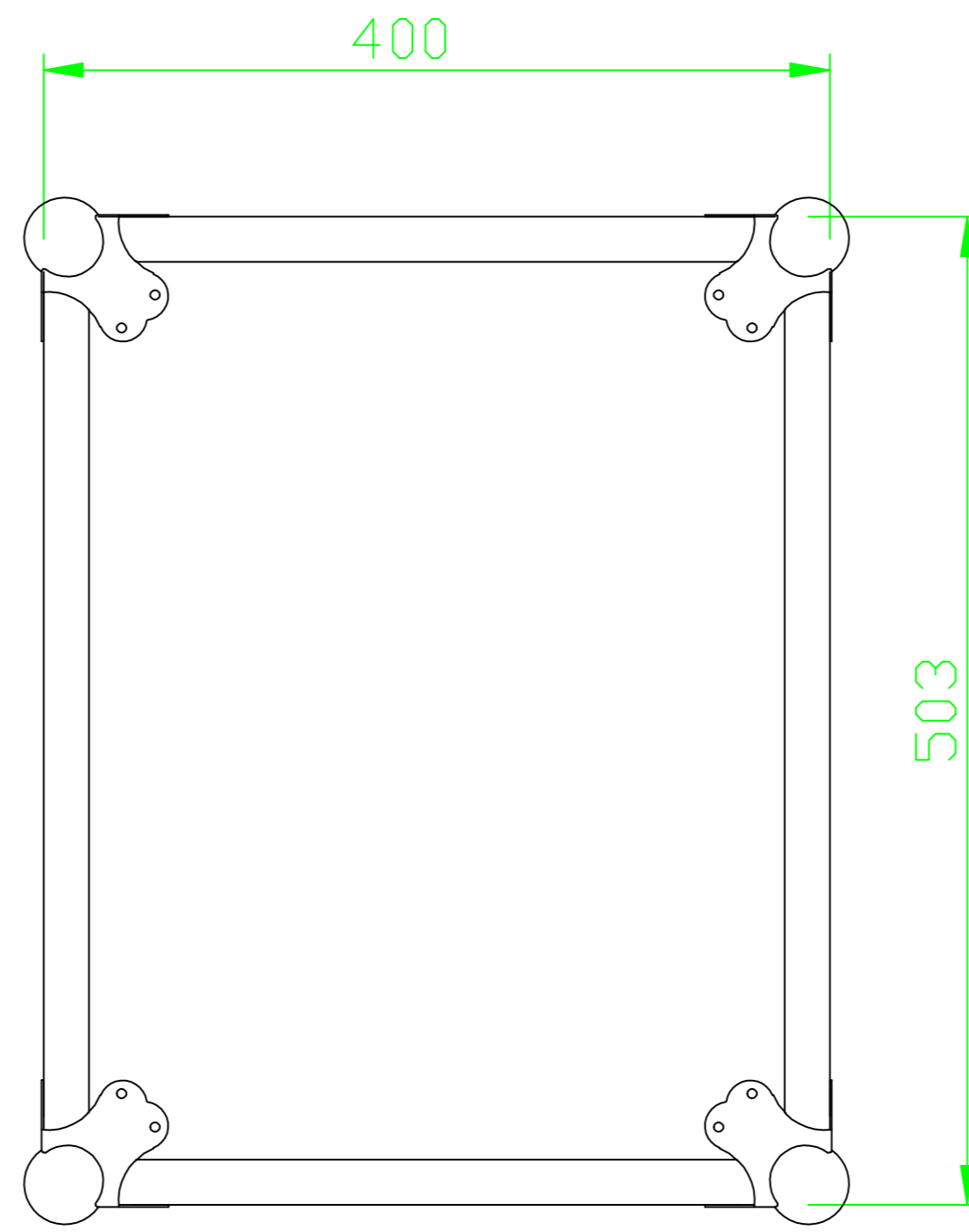
top view
