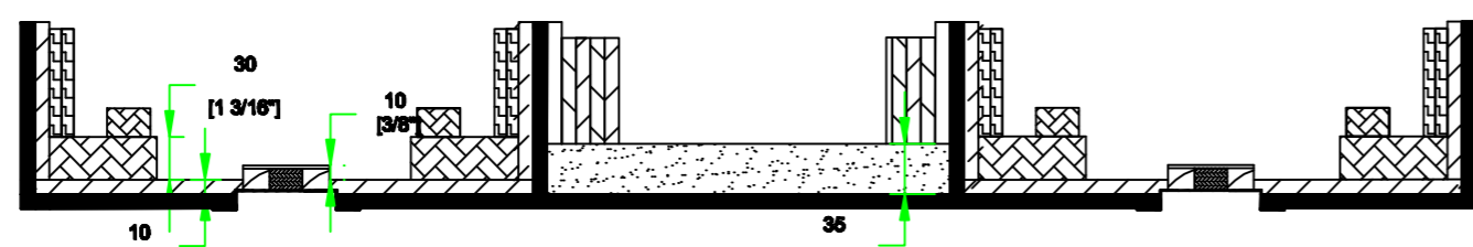
C-C VIEW
