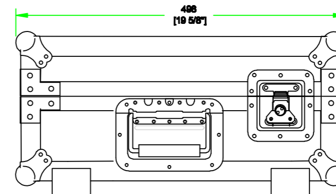
LEFT VIEW
