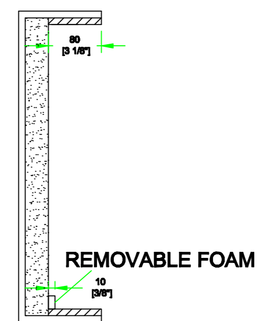
F-F VIEW
