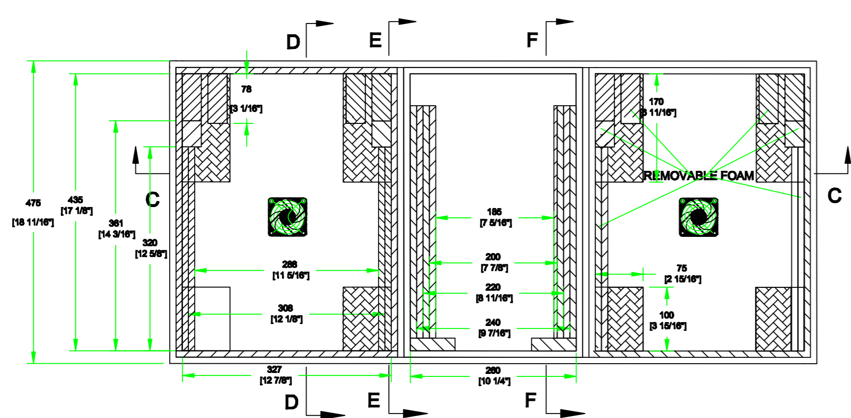
TOP VIEW OF BASE
