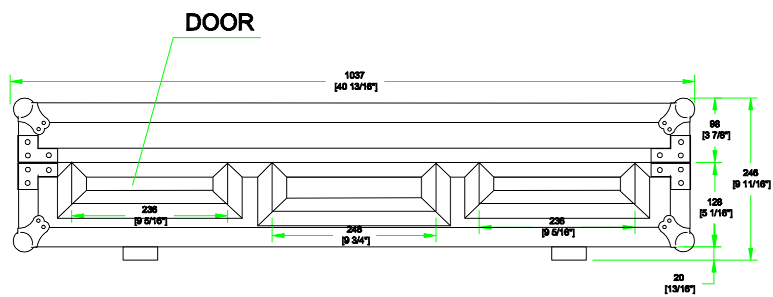
FRONT VIEW
