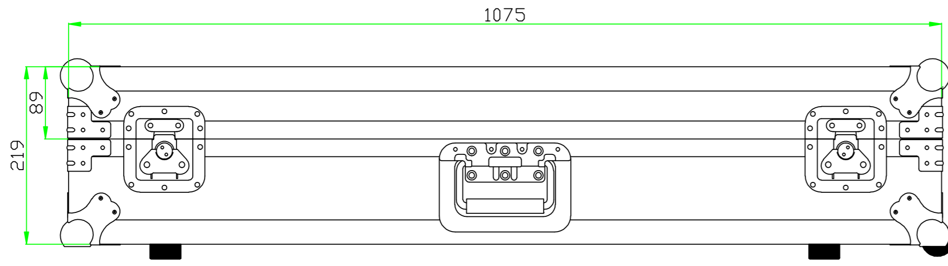
BACK VIEW
