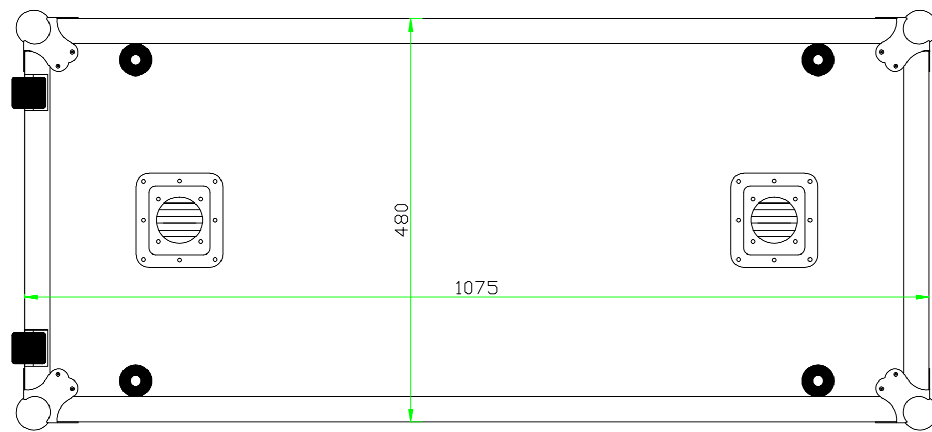
BOTTOM VIEW
