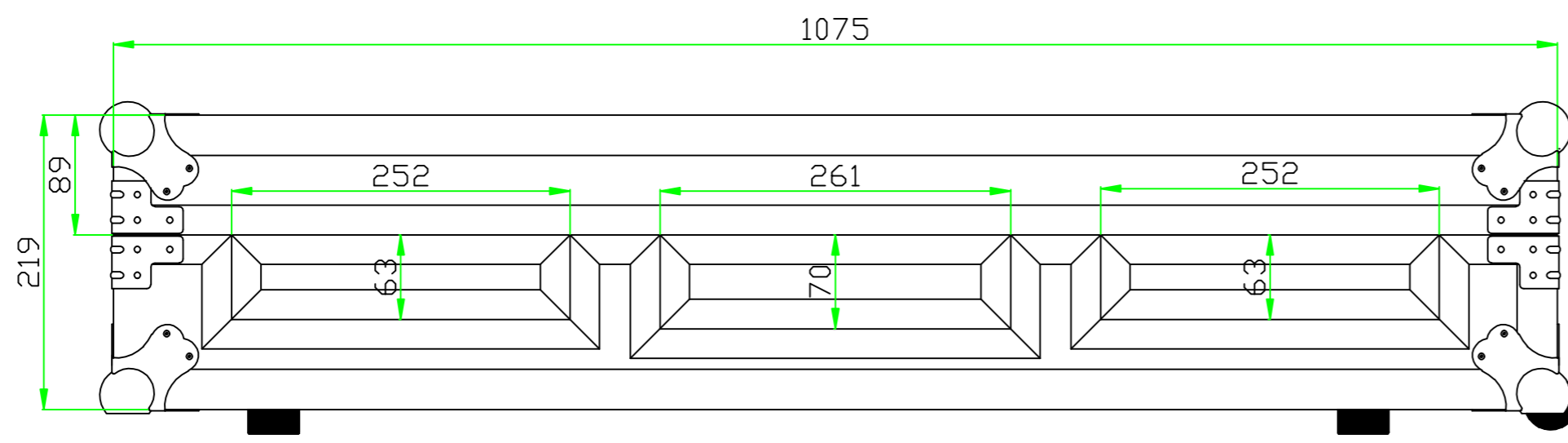
FRONT VIEW
