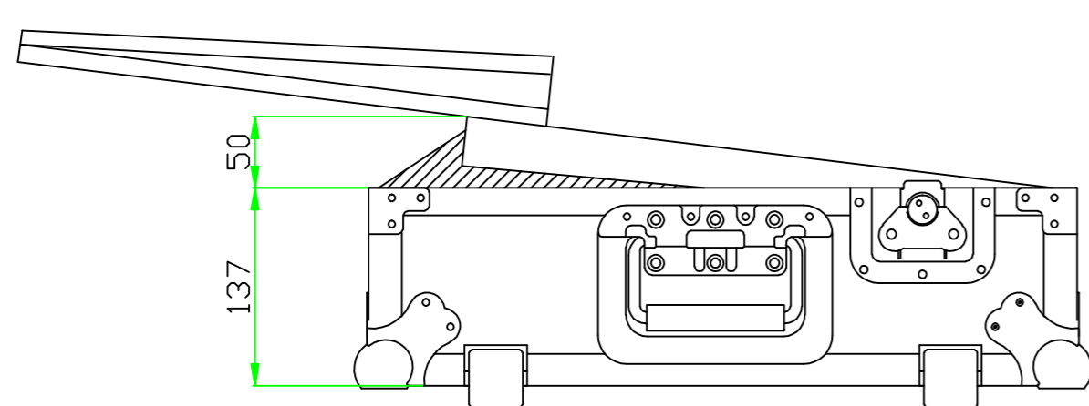
LEFT VIEW
