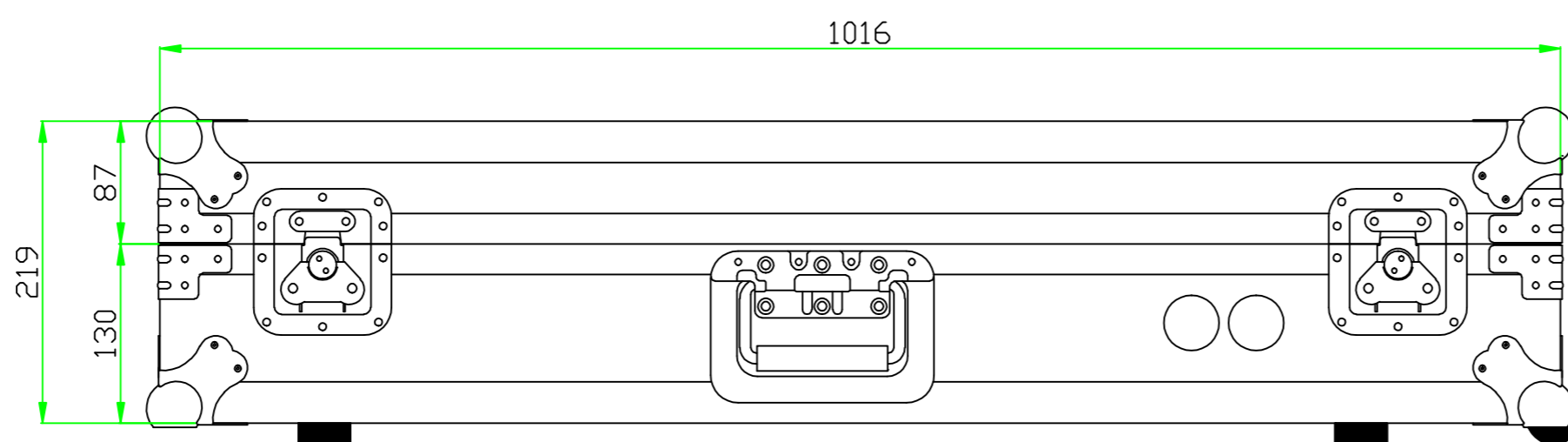
BACK VIEW
