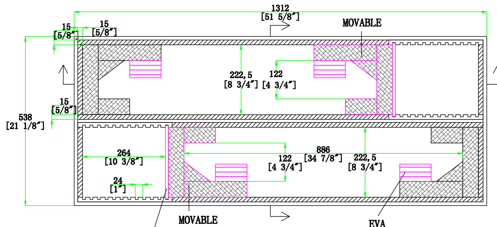
TOP VIEW OF BASE
