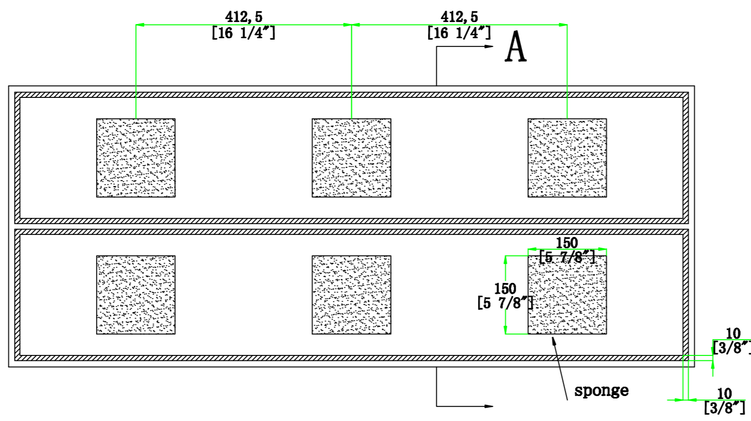
BOTTOM VIEW OF COVER
