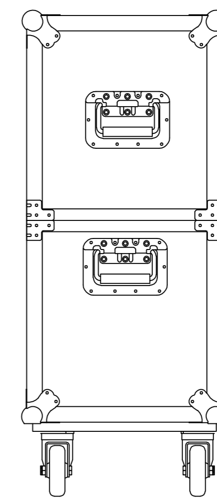
LEFT & RIGHT VIEW
