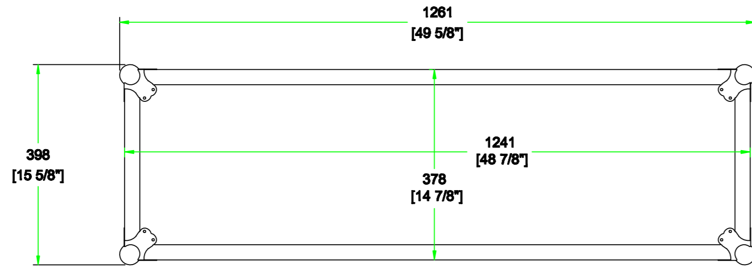
TOP VIEW
