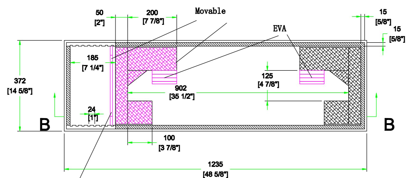
INSIDE VIEW OF BASE
