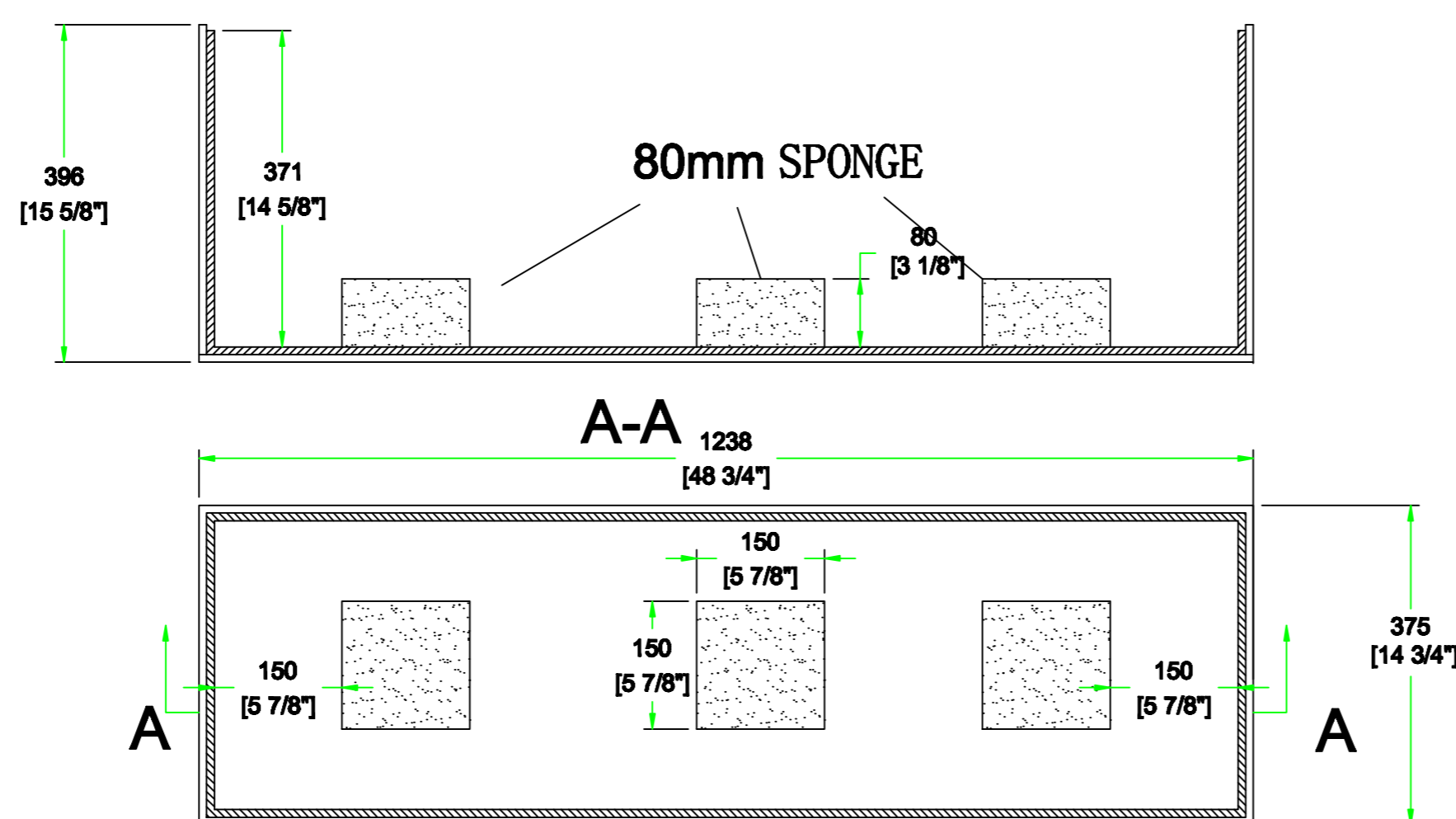
INSIDE VIEW OF COVER
