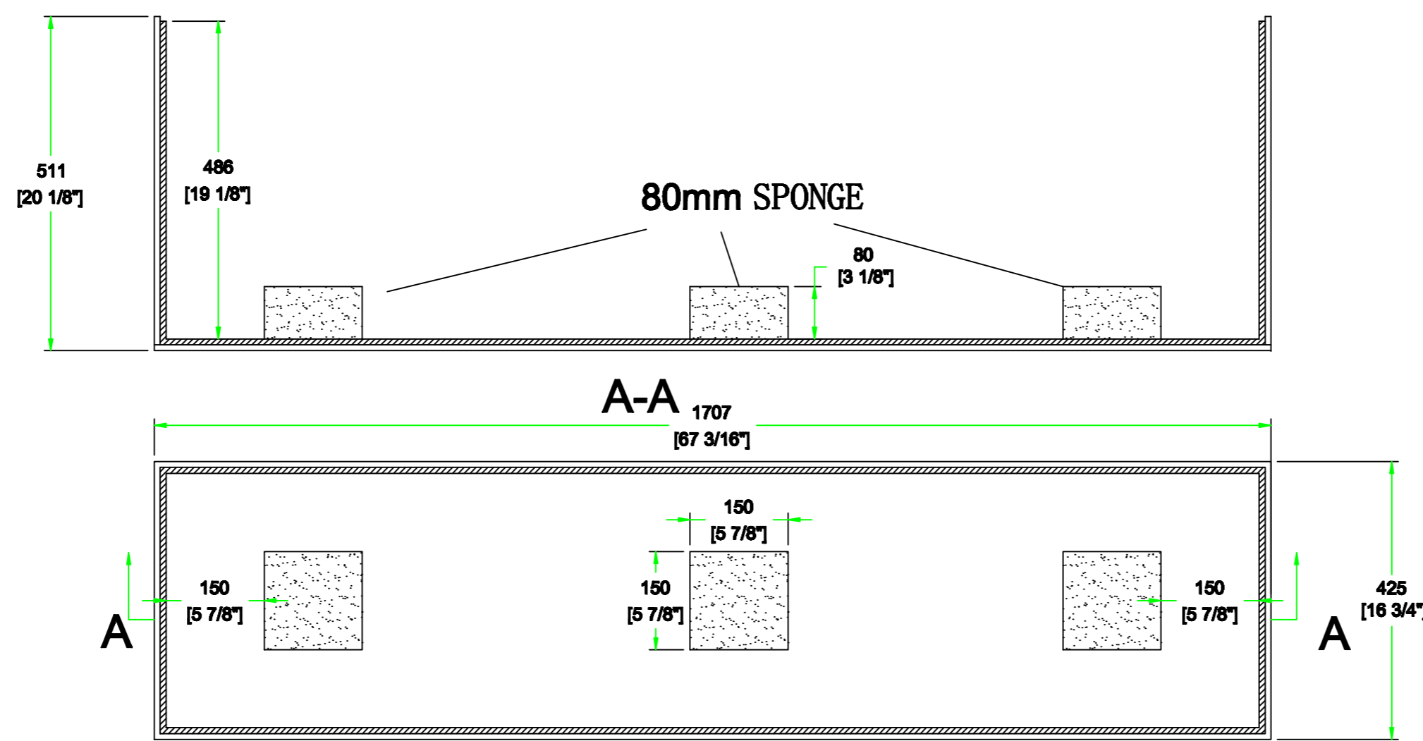
INSIDE VIEW OF COVER
